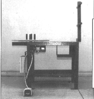
SIDEWALL STRIP APPLICATOR 10/16
